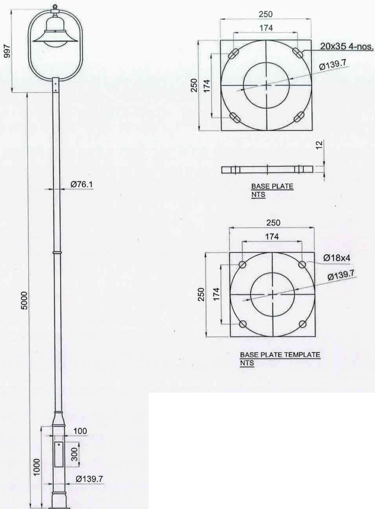
POLE BLENHEIM 5M WITH VALE POST TOP – (ITEM NO.2)
