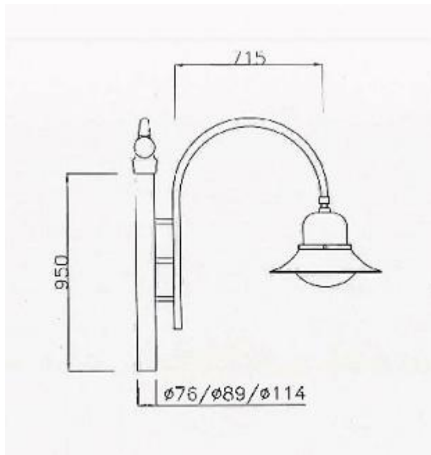
CASCADE BRACKET 0.7M SOH WITH VALE – (ITEM NO.10)
