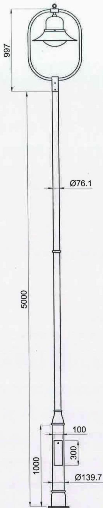
POLE BLENHEIM 5M WITH VALE POST TOP – (ITEM NO.2)
