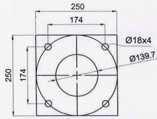
BASE PLATE TEMPLATE NTS
