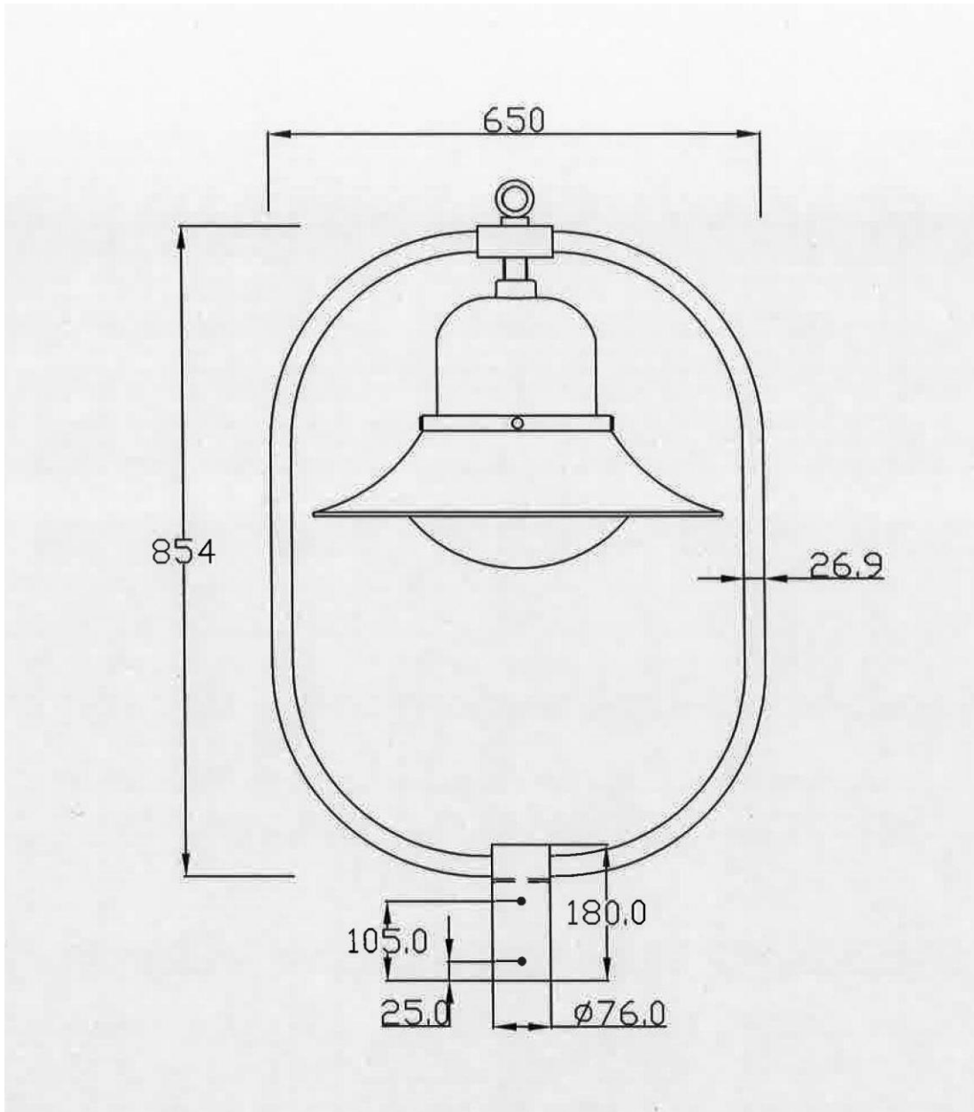
POST TOP WITH BRACKET – (ITEM NO.1)
